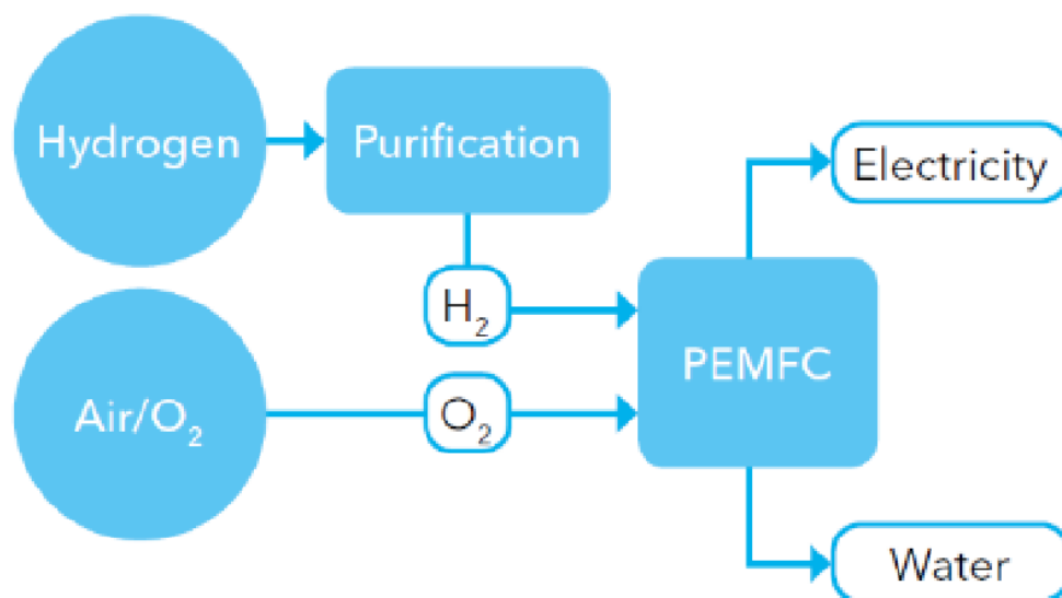
Figur 8-1: Prinsippkisse for PEM-brenselceller (DNV GL, 2017).
